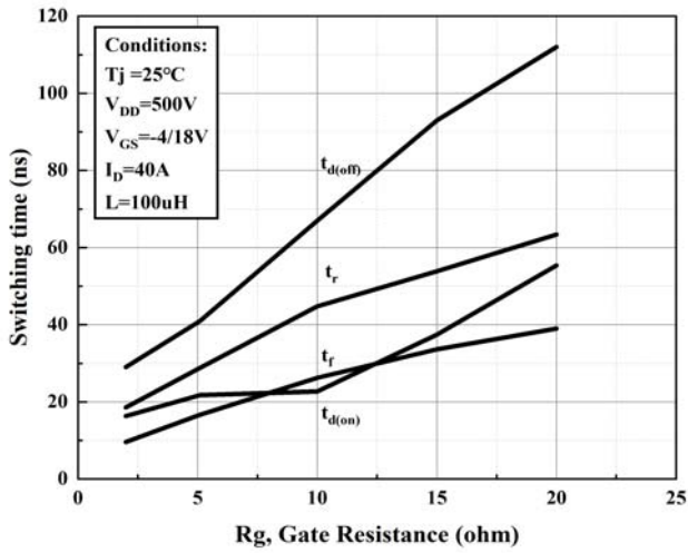
Figure 21. Switching Times vs. R_g
