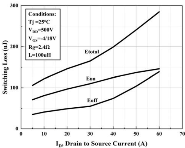
Figure 19. Clamped Inductive Switching Energy vs. Drain Current
