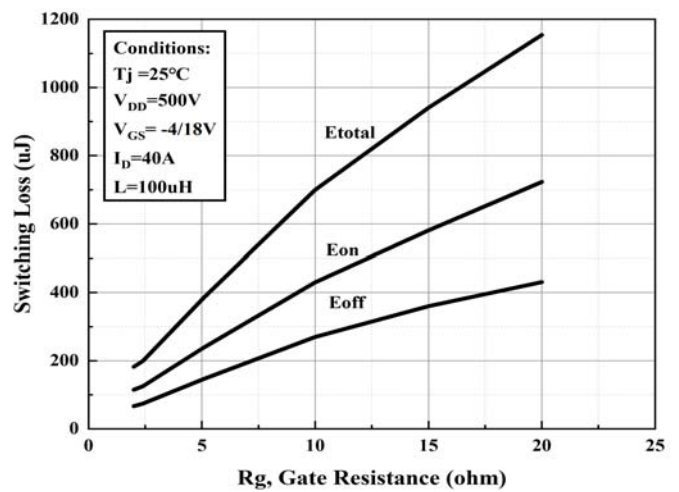
Figure 20. Clamped Inductive Switching Energy vs. R g
